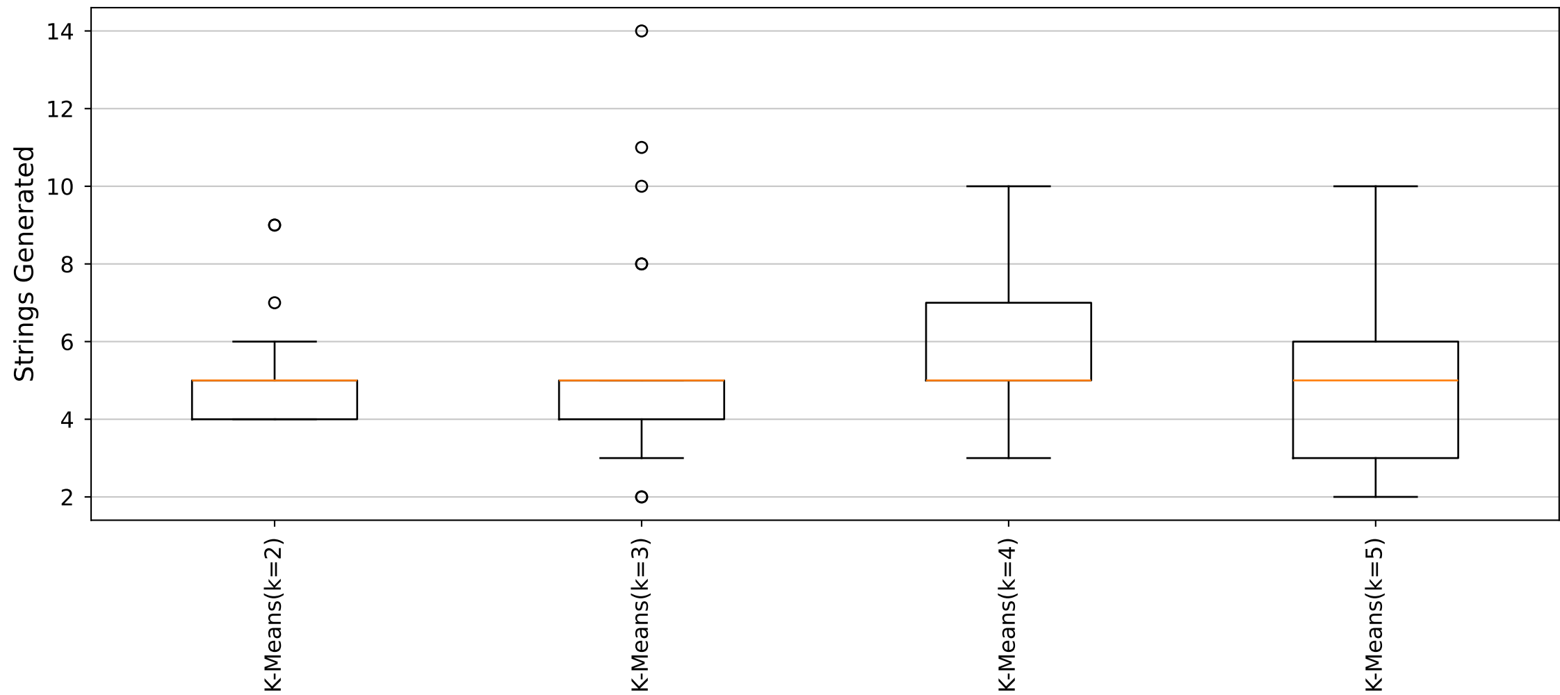
YARA Rules Strings Generated Distribution (Cluster35_Size5 dataset)
